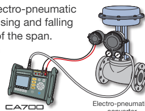
CA700 Electro-pneumatic converter
