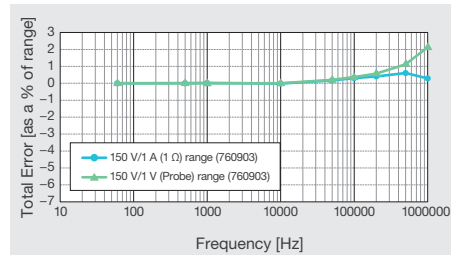
Frequency versus power accuracy at zero power factor
